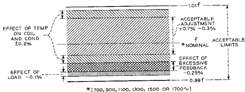
Fig. 12 — Frequency of output with effect of various factors that may alter the frequency indicated.
