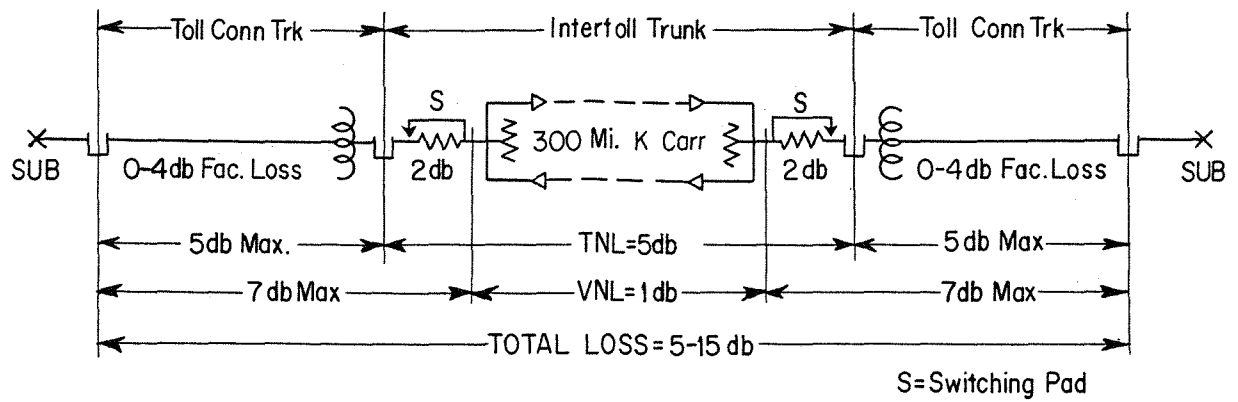
Fig.A-Intertoll Trunks Terminated at Terminal Net Loss
