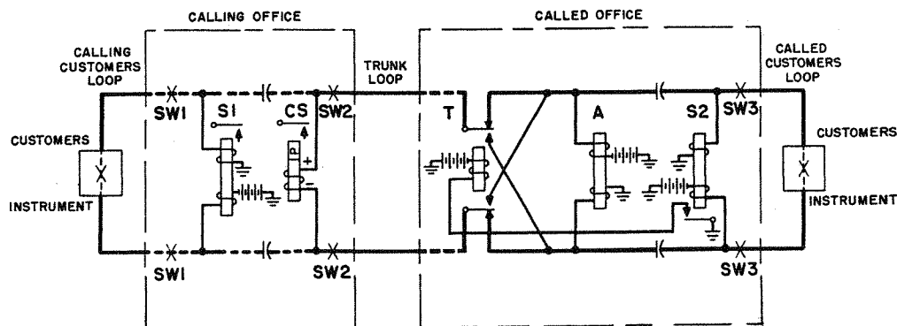
Fig. 4 - Reverse Battery Supervision
