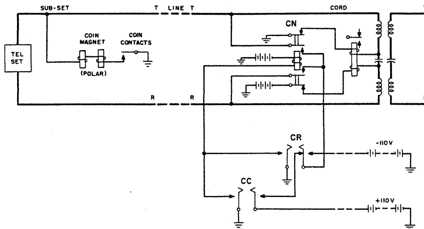
FIG 15 - COIN COLLECT AND RETURN CIRCUIT
