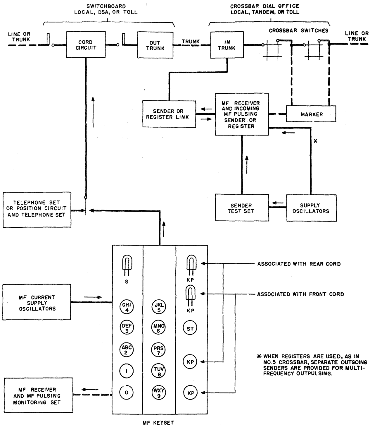
FIG.12-PLAN OF MF PULSING SYSTEM
