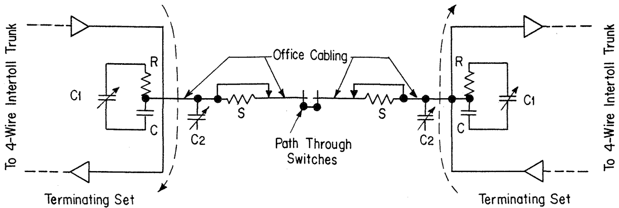
Fig.A—Switching Pads Employed
