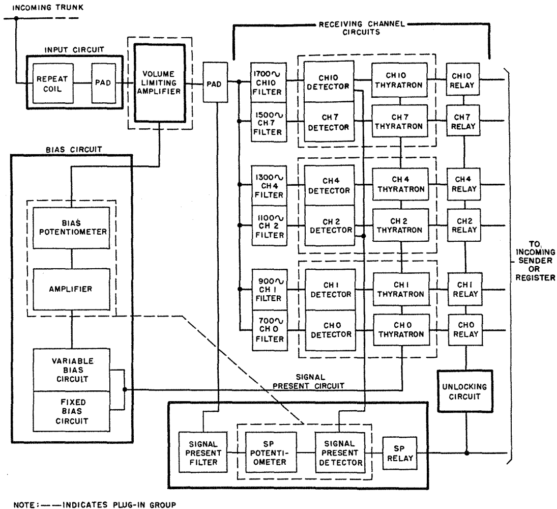
FIG. 13 - MF RECEIVER PLAN
