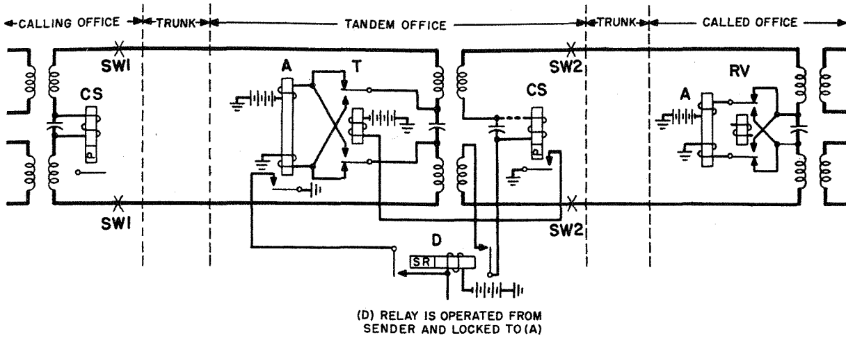
FIG. 5 - REPEATED REVERSE BATTERY SUPERVISION
