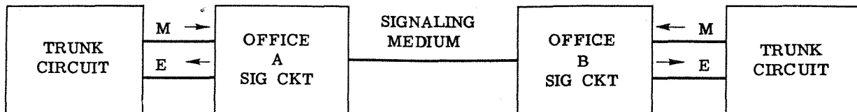
Fig. 7 - E and M Lead Control
