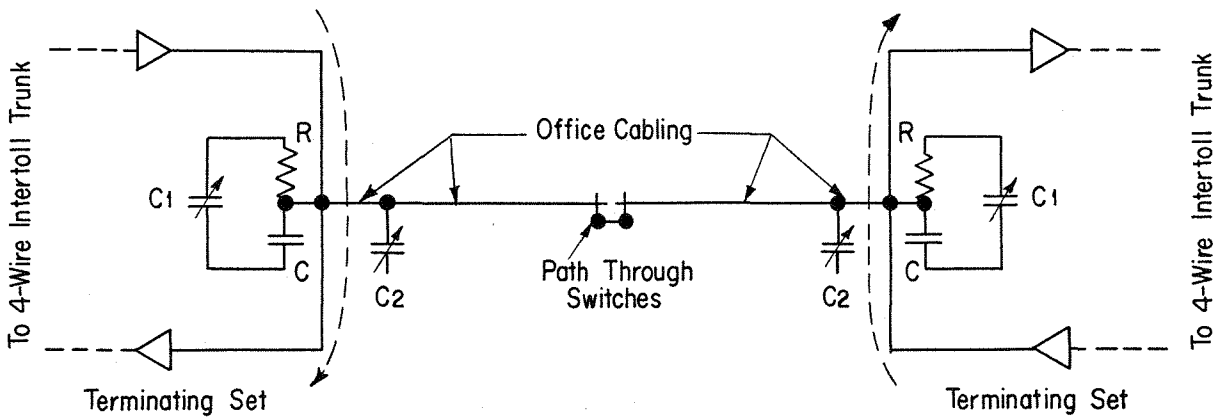
Fig.B—No Switching Pads Employed
