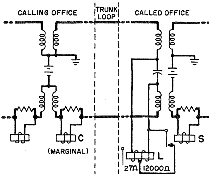
FIG. 6 - HIGH-LOW SIGNALING
