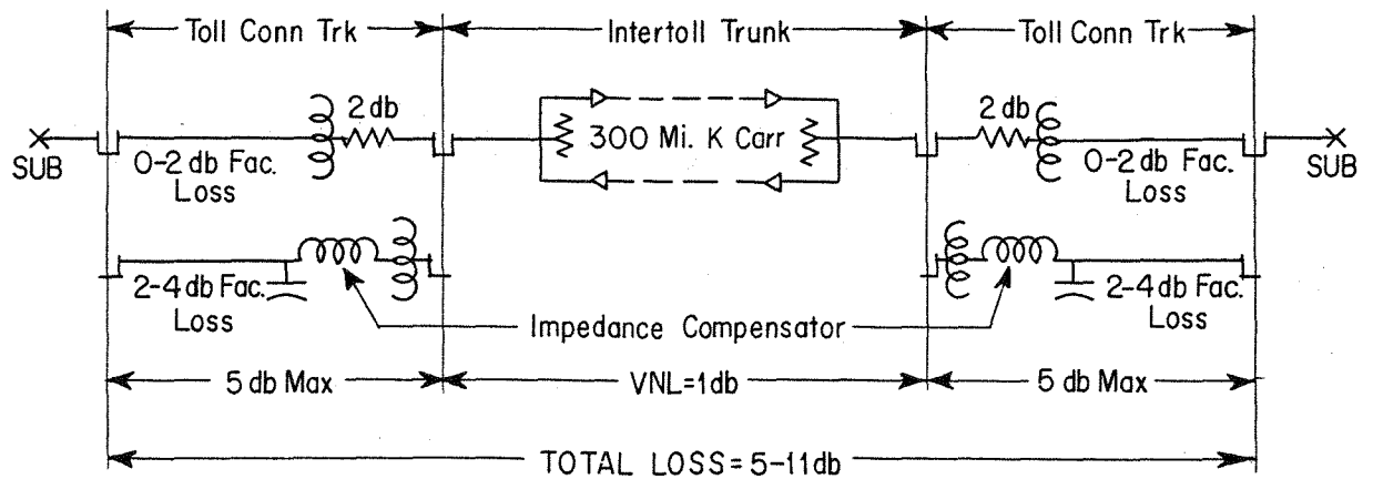
Fig.B-Intertoll Trunks Terminated at Via Net Loss
