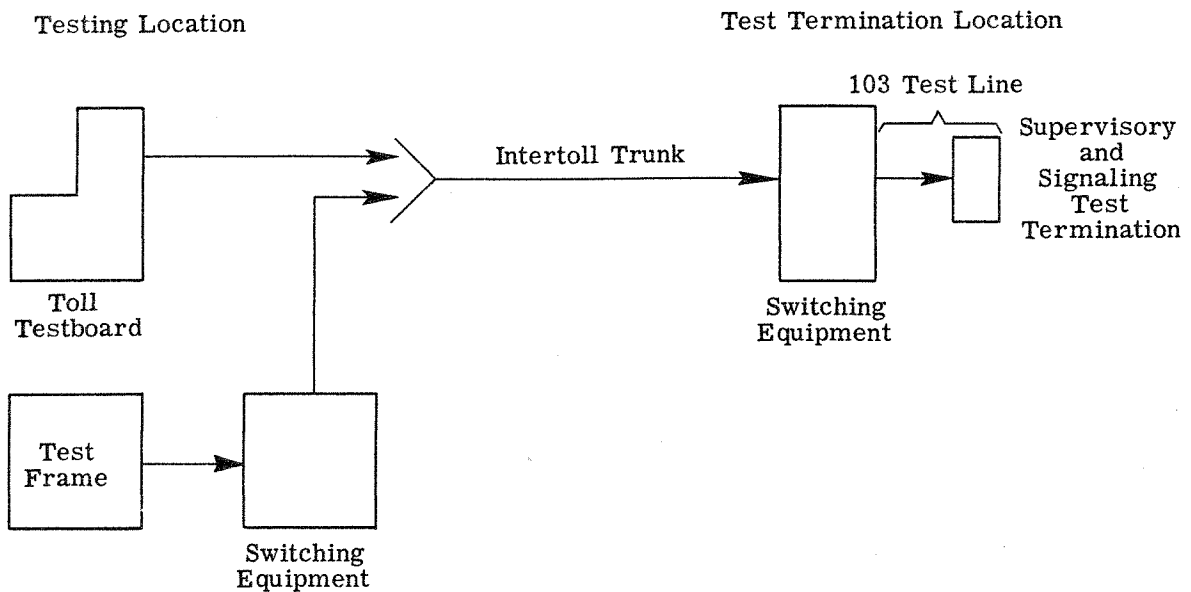
Fig. 4. Arrangement For Code 103 Test Line
