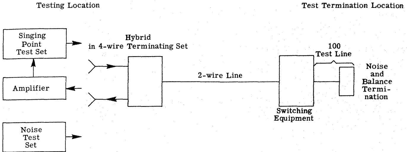
Fig. 1. Arrangement For Code 100 Test Line
