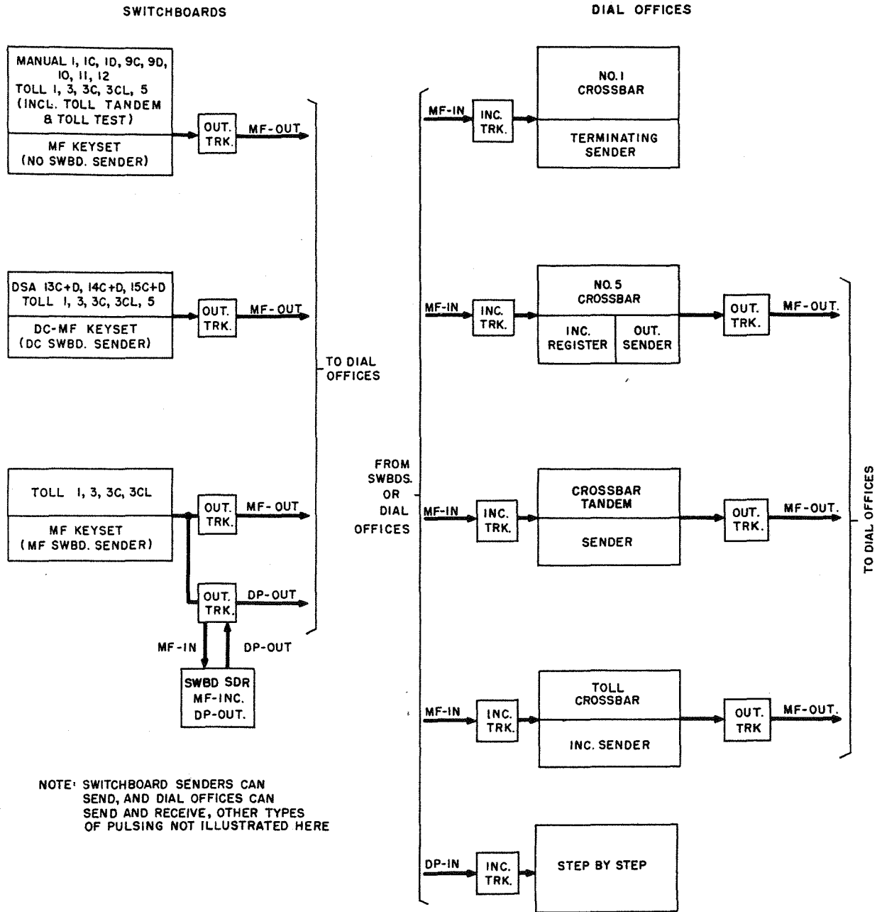
FIG. 14—APPLICATION PLAN OF MF PULSING SYSTEM
