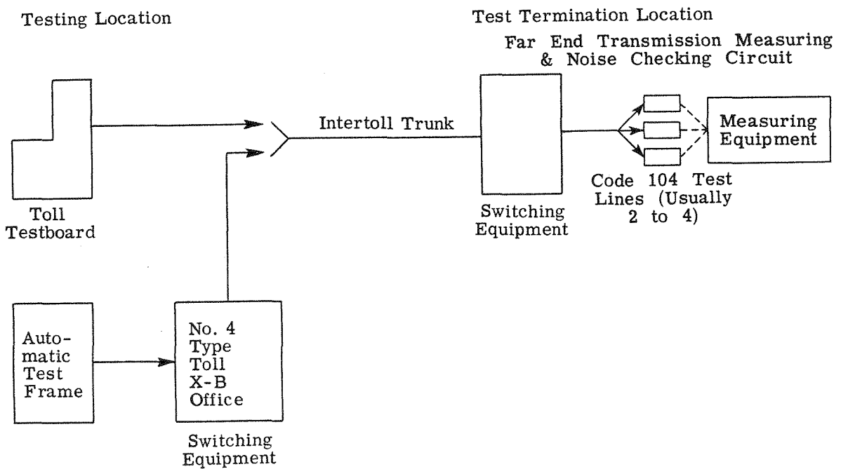
Fig. 5. Arrangement For Code 104 Test Line
