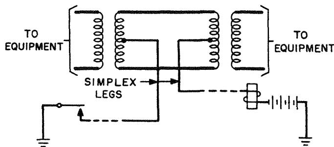
Fig. 10 - Simplex Signaling
