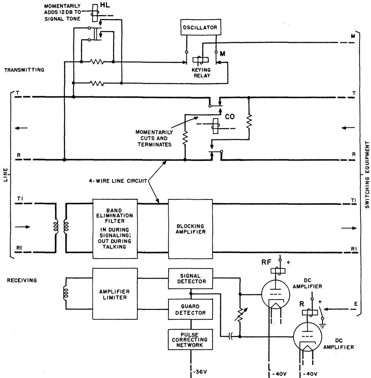
FIG.11 - SIMPLIFIED SCHEMATIC DRAWING OF THE SF CIRCUITS AS CONNECTED TO A FOUR-WIRE TRANSMISSION CHANNEL
