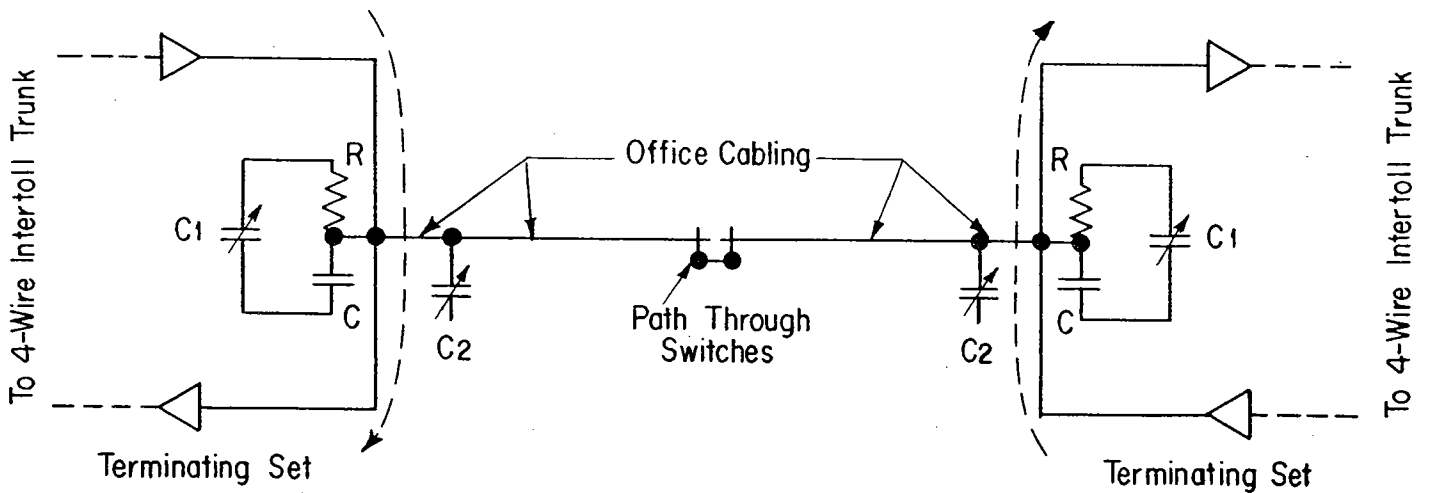
Fig. B—No Switching Pads Employed
