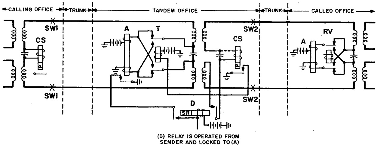
FIG. 5 - REPEATED REVERSE BATTERY SUPERVISION
