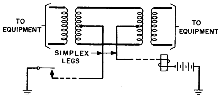
FIG. 9 - SIMPLEX SIGNALING
