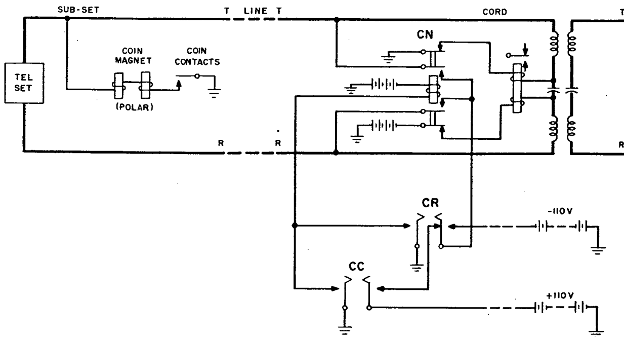
FIG. 14 - COIN COLLECT AND RETURN CIRCUIT
