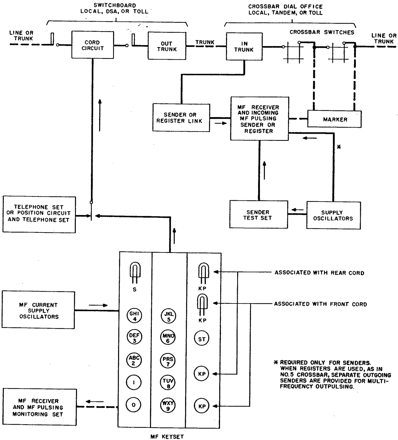
FIG. II - PLAN OF MF PULSING SYSTEM
