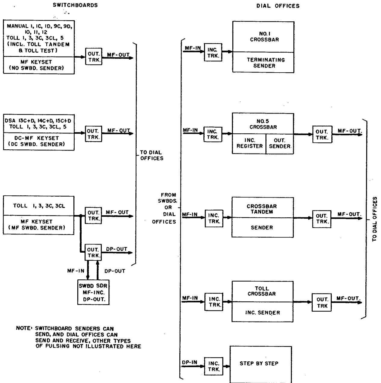
FIG. 13—APPLICATION PLAN OF MF PULSING SYSTEM
