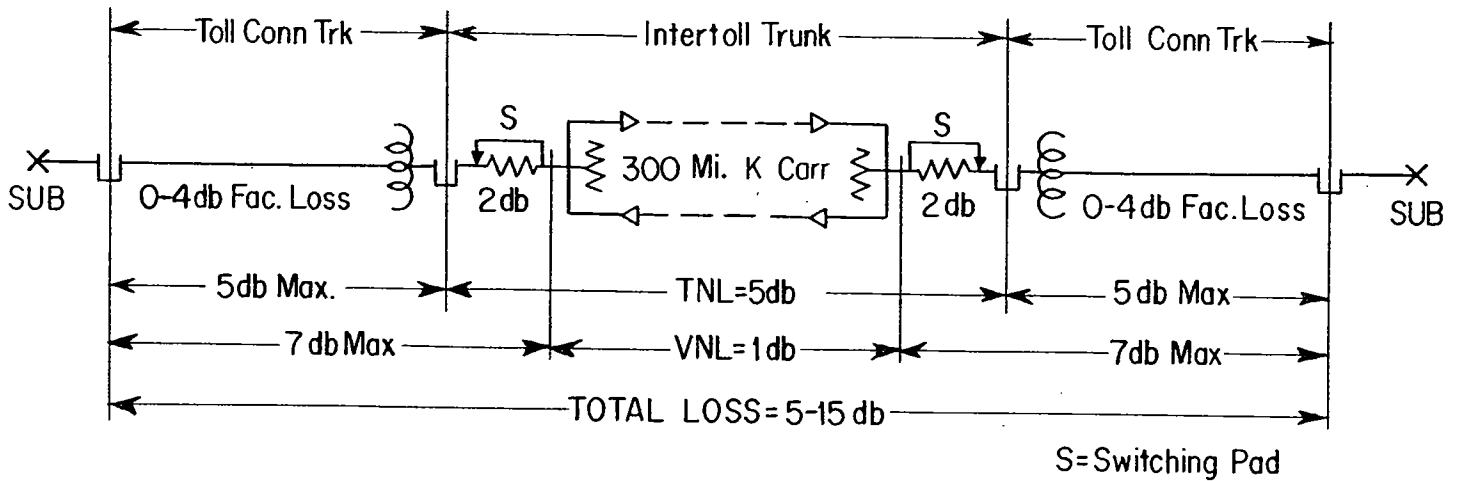
Fig.A-Intertoll Trunks Terminated at Terminal Net Loss
