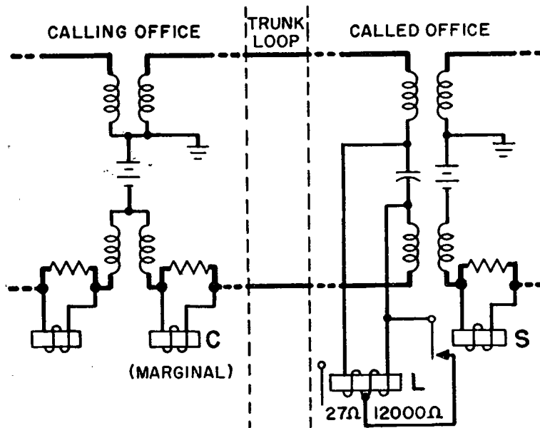
FIG. 6 - HIGH-LOW SIGNALING
