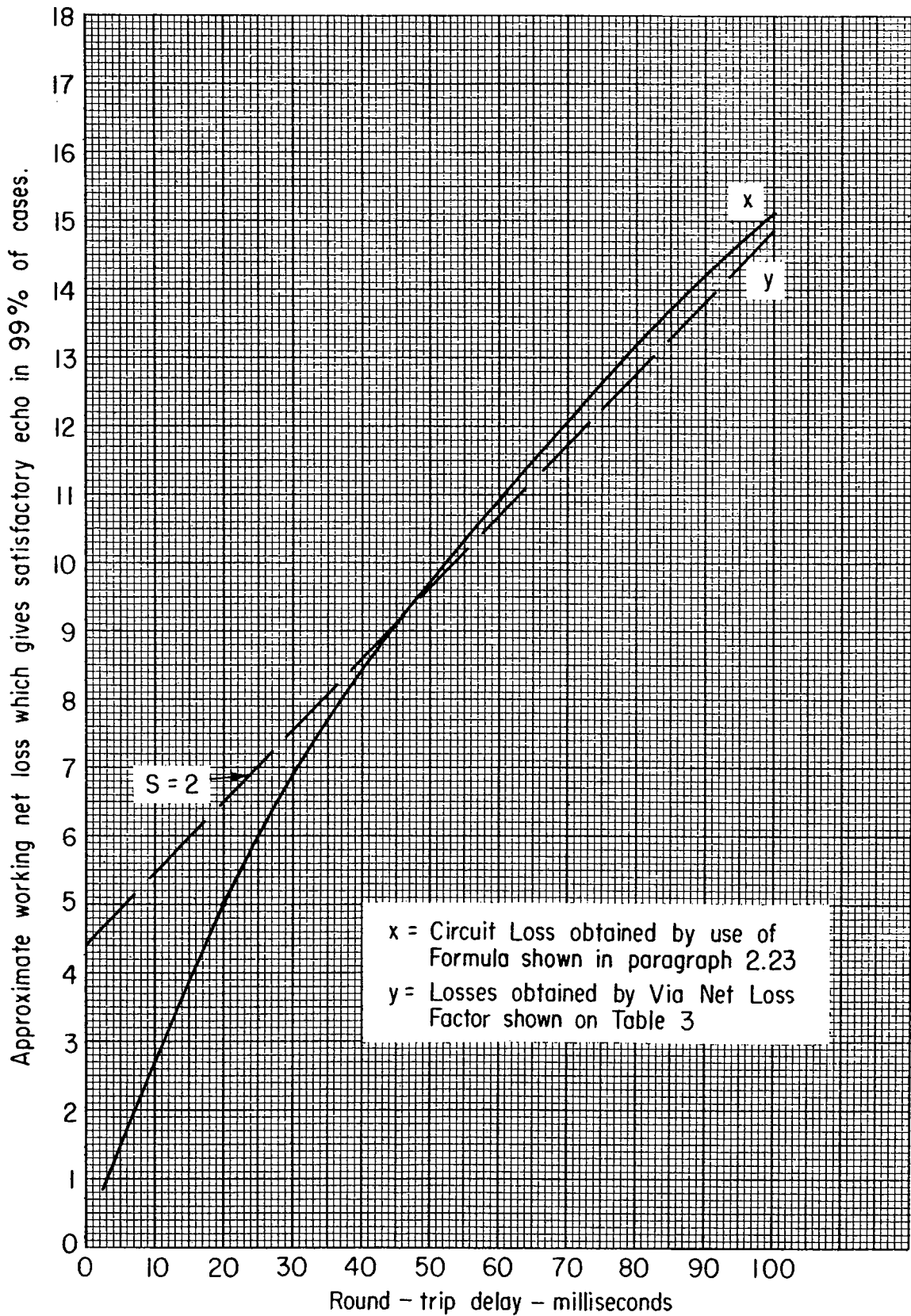
APPROXIMATE RELATIONSHIP BETWEEN ROUND-TRIP DELAY AND PERMISSIBLE WORKING ONE-WAY LOSS FOR AN INTERTOLL TRUNK FROM ECHO STANDPOINT FOR 4-WIRE CIRCUITS AND 4-WIRE SWITCHING.
