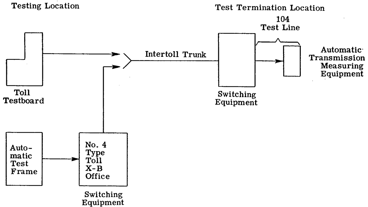
Fig. 5. Arrangement For Proposed Code 104 Test Line
