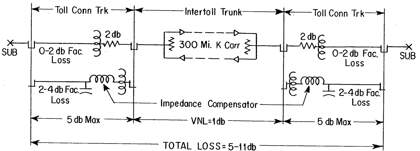
Fig.B-Intertoll Trunks Terminated at Via Net Loss
