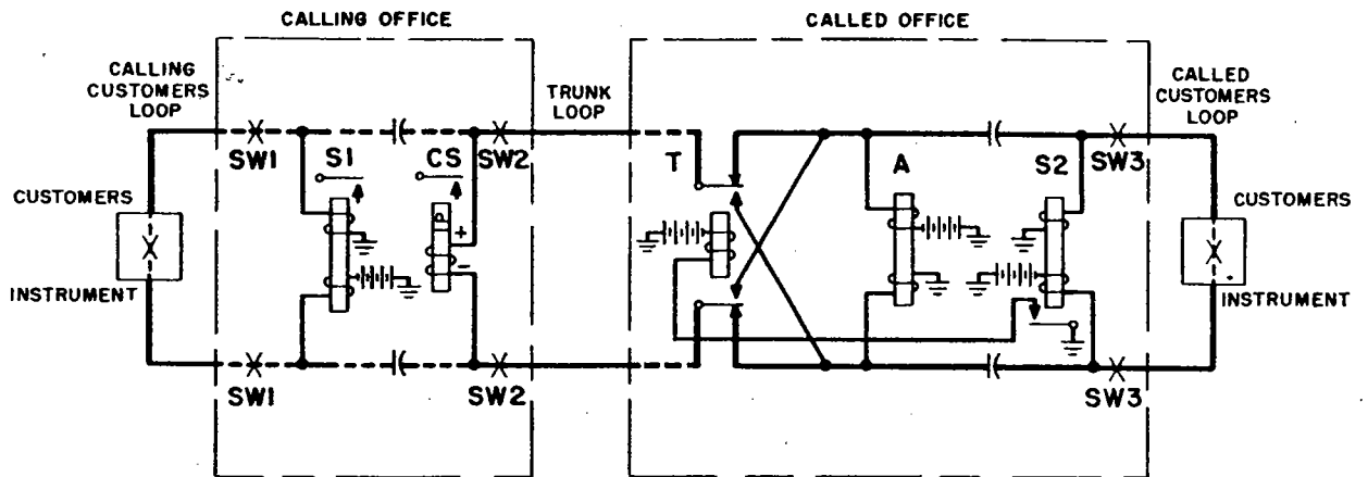
FIG. 4 - REVERSE BATTERY SUPERVISION
