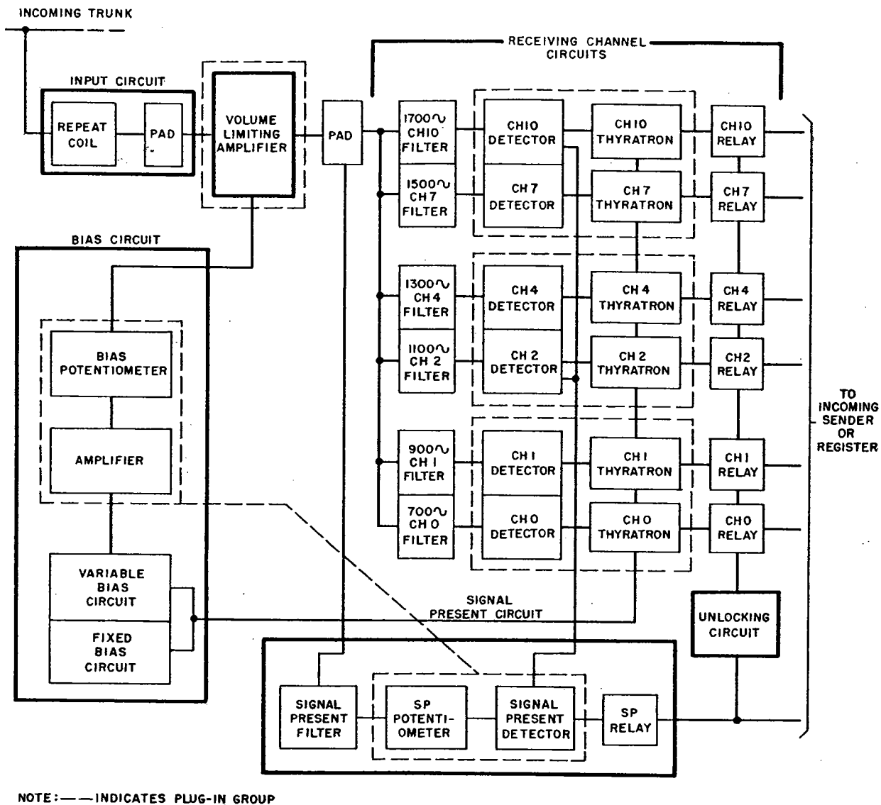
FIG.12- MF RECEIVER PLAN
