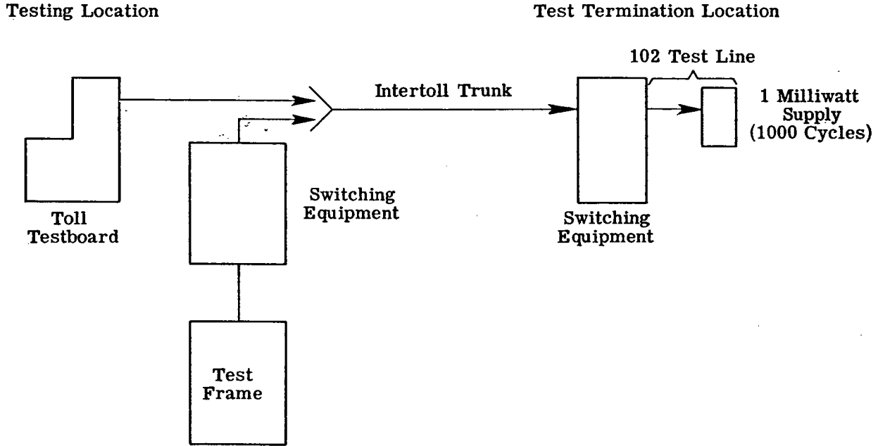
Fig. 3. Arrangement For Code 102 Test Line
