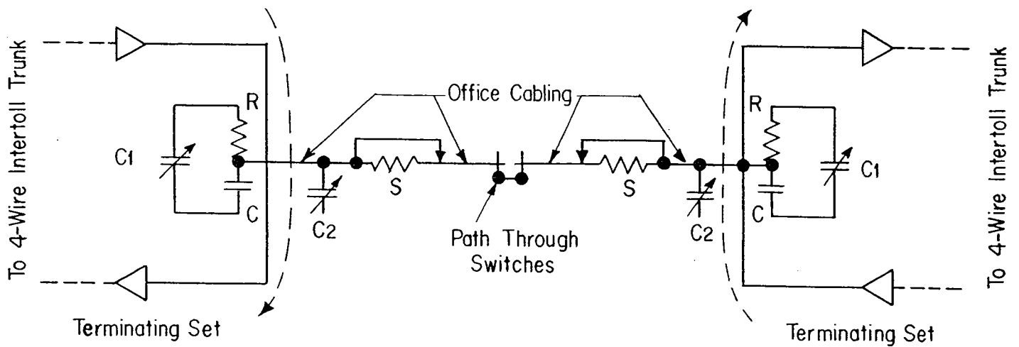
Fig. A—Switching Pads Employed
