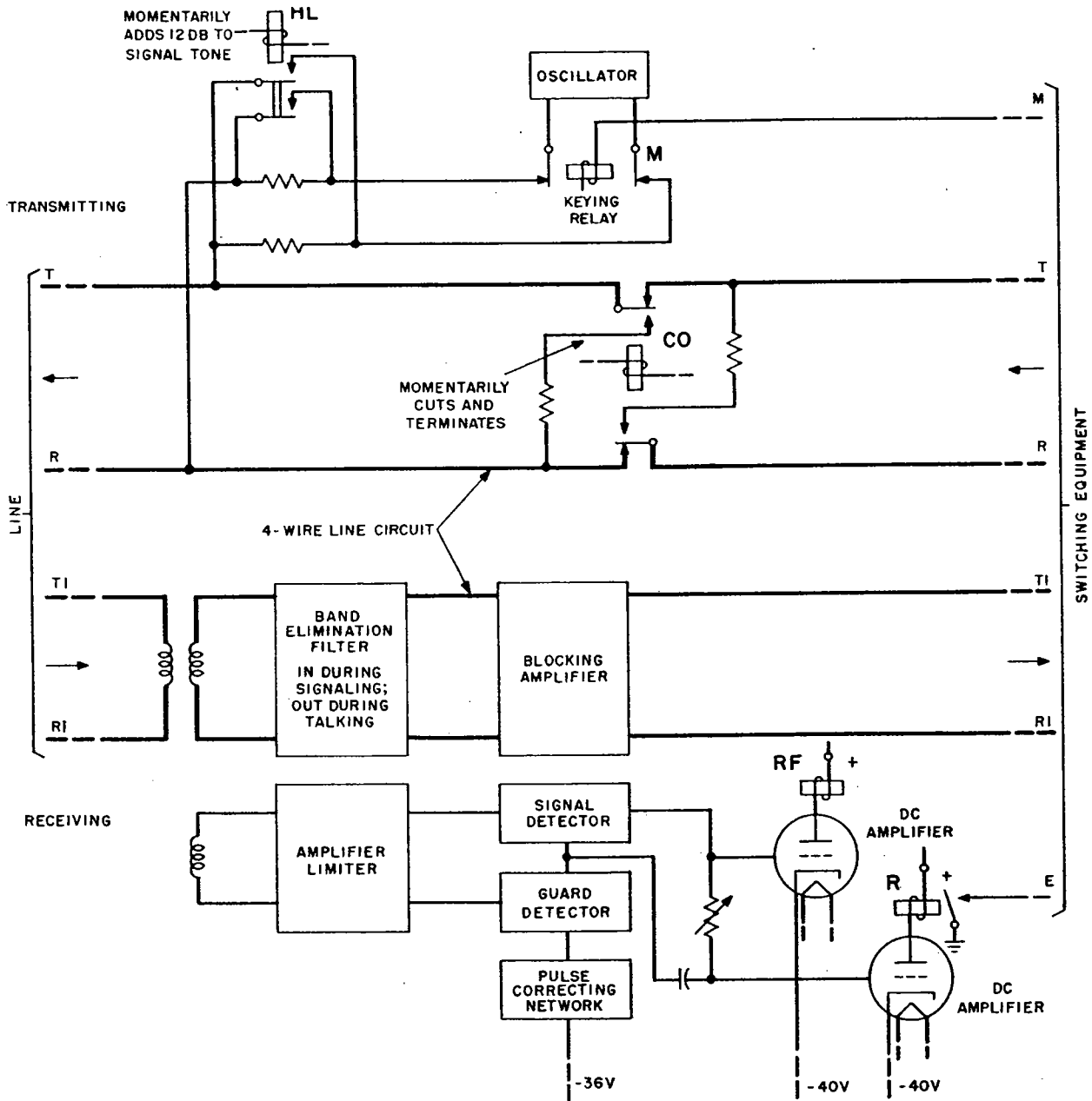
FIG.10 - SIMPLIFIED SCHEMATIC DRAWING OF THE SF CIRCUITS AS CONNECTED TO A FOUR-WIRE TRANSMISSION CHANNEL
