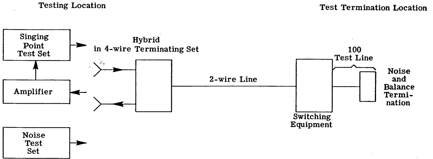
Fig. 1. Arrangement For Code 100 Test Line
