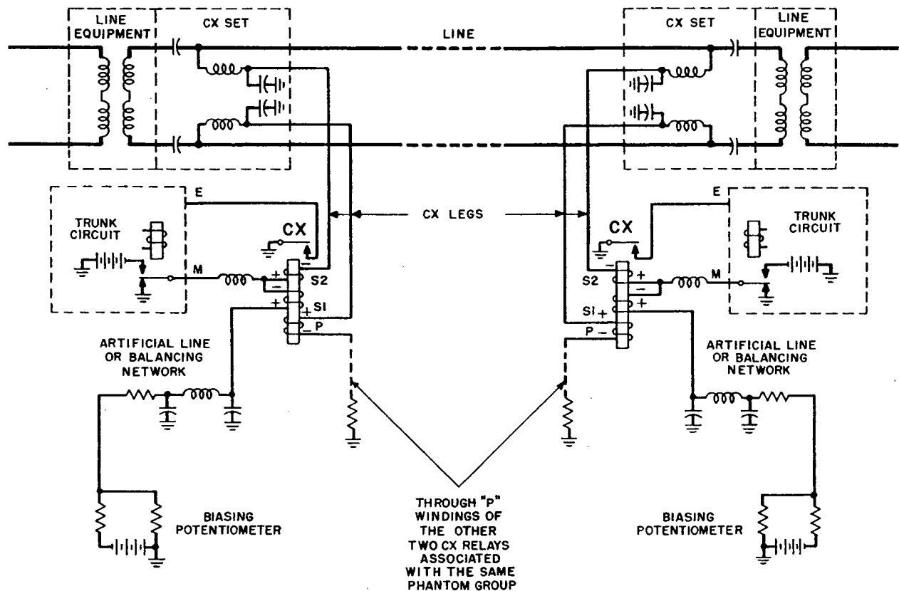
FIG. 8 - COMPOSITE SIGNALING CIRCUIT FOR ONE VOICE CHANNEL
