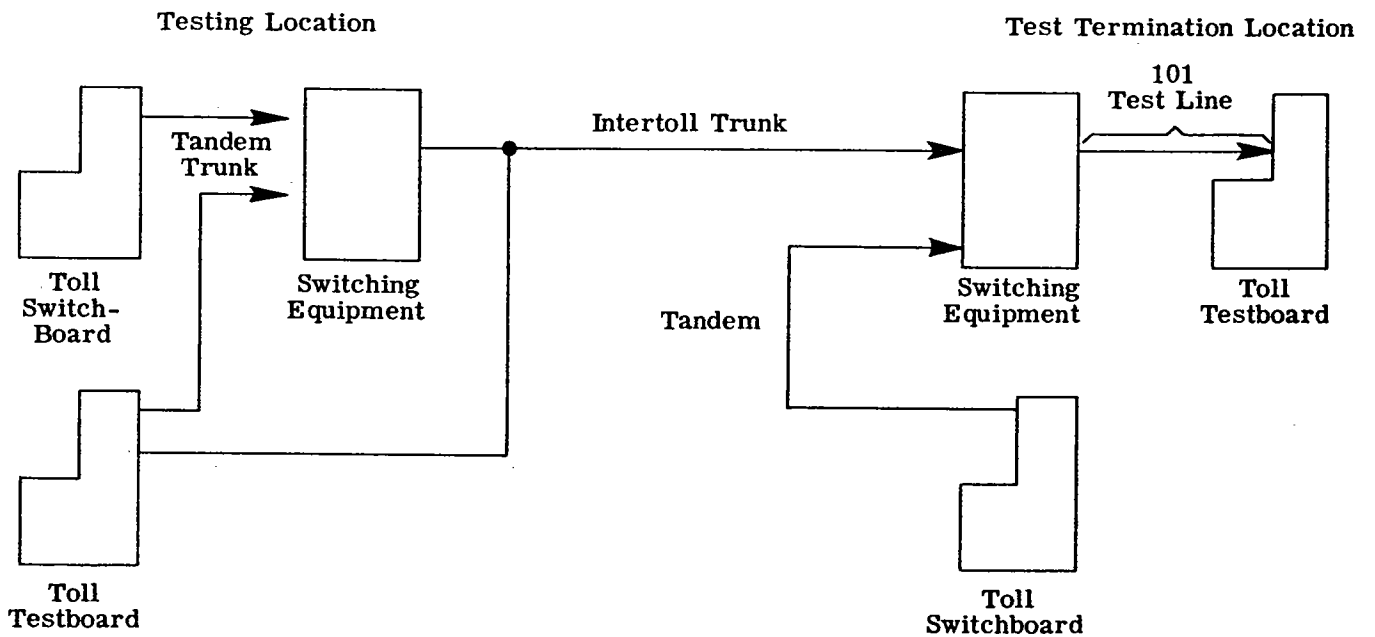
Fig. 2. Arrangement For Code 101 Test Line
